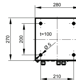
ELECTRONIC BOX (DRILLING PATTERN)
